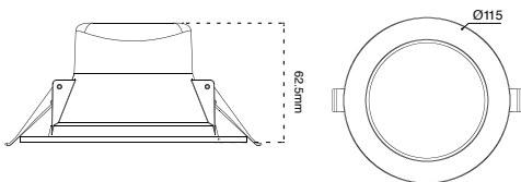
CUT-OUT: Ø90mm
