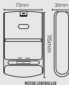
MOTOR CONTROLLER
